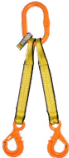
SYNTHETIC LIFTING BRIDLE WITH X100 FITTINGS
